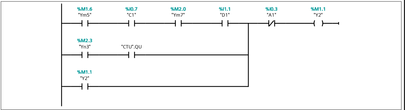
Network 13: A
