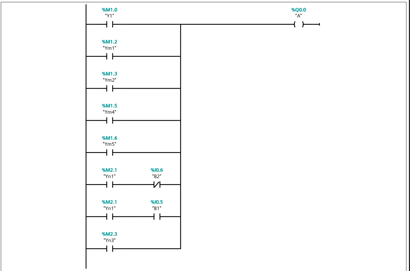
Network 14: B
